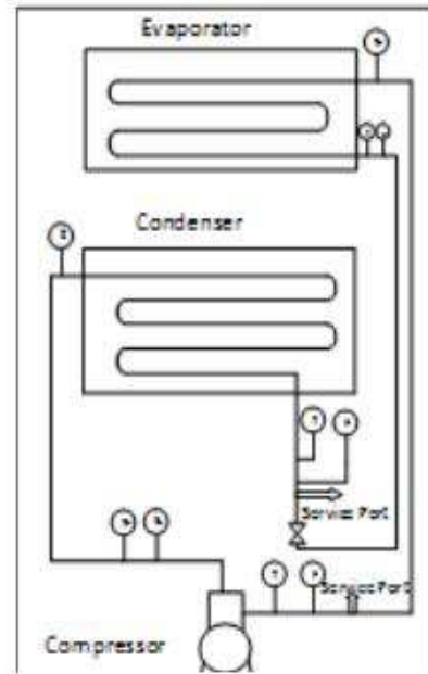
Fig. 1: Experimental Setup of the Investigation Unit and Apparatus & Fig. 2: Schematic Diagram of the Investigation Unit and Apparatus
