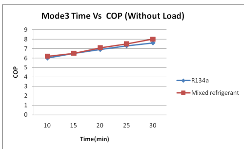
Fig. 5: Mode 3 Time Vs COP (Without Load)
