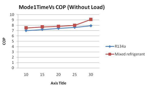
Fig. 3: Mode 1 Time Vs COP (Without Load)
