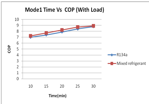
Fig. 7: Mode 1 Time Vs COP (With Load)
