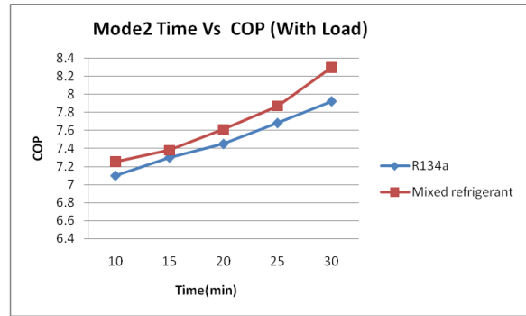
Fig. 8: Mode 2 Time Vs COP (With Load)
