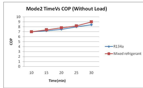
Fig. 4: Mode 2 Time Vs COP (Without Load)
